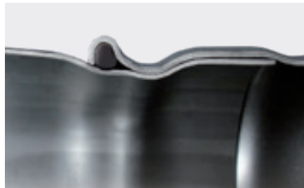
The Geberit pressing tool ensures permanently reliable connections.
