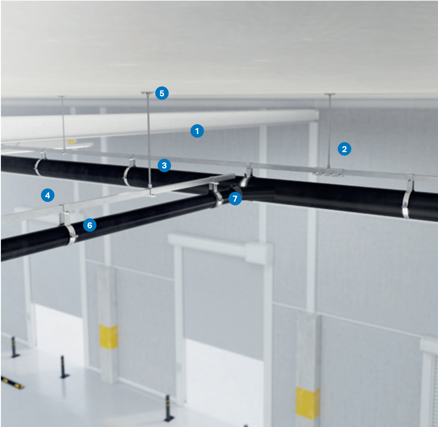
Fastening with square profiles for pipes d40–d200
