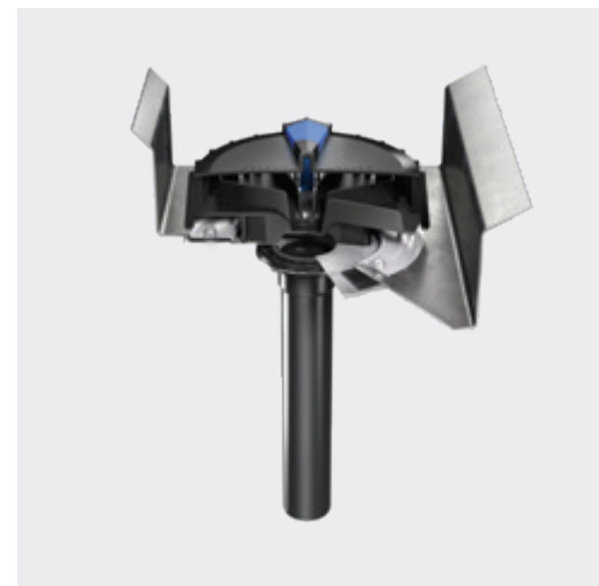
EXAMPLE 4: ROOF WITH STEEL GUTTER Thanks to its compact design, Geberit Pluvia is also suitable for installation in gutters. Depending on the product material, the system can be installed using soldering or by means of a flange.
