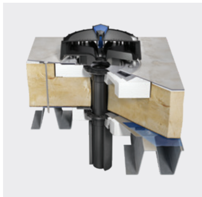
EXAMPLE 2: LIGHTWEIGHT ROOF, INSULATED WITH ROOF FOIL AND THE GEBERIT VAPOUR BARRIER CONNECTION Lightweight roofs benefit from the low static load thanks to Geberit Pluvia. The installation is performed with a flange connection, allowing the long connection pipe to effortlessly overcome high insulation thicknesses. The Geberit vapour barrier connection can be used both for foil and bitumen.
