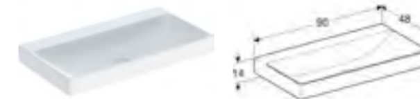
90cm washbasin classic waste H 14 / W 90 / D 48cm
