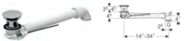
Geberit waste outlet, space-saving model, slim design, with external waste plug and lever actuation: G=1 1/4"
