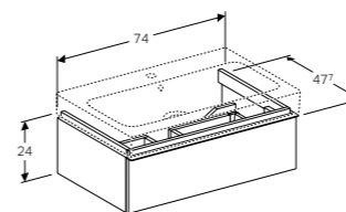
Cabinet for 75cm washbasin, with one drawer W 74 / D 47.7 / H 24cm
