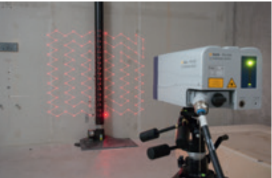
Non-contact and full-surface vibration measurement.
