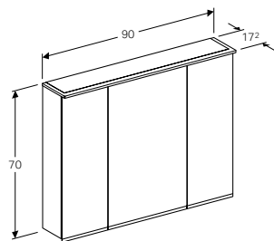
90cm option plus mirror cabinet with functional and ambient lighting, three doors W 90 / D 17.2 / H 70cm
