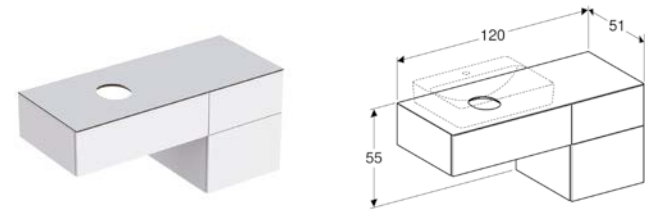
120cm cabinet for lay-on washbasin, with three drawers W 120 / D 51 / H 55cm With integrated shelf surface and trap.
