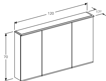
120cm option plus mirror cabinet with functional and ambient lighting, three doors W 120 / D 17.2 / H 70cm
