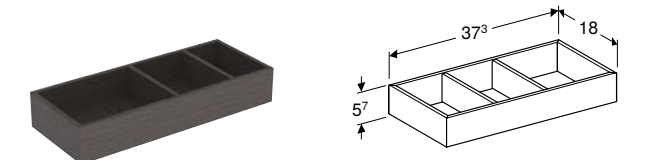
Square drawer insert low W 18 / D 37.3 / H 5.7cm H-partition suitable for VariForm units.
