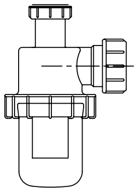
152.090.16.1 TRAP + 152.095.00.1 0.6 LTR. GLASS RECEIVER
